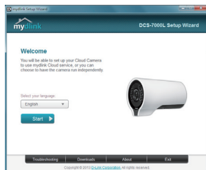
SetupWizard
