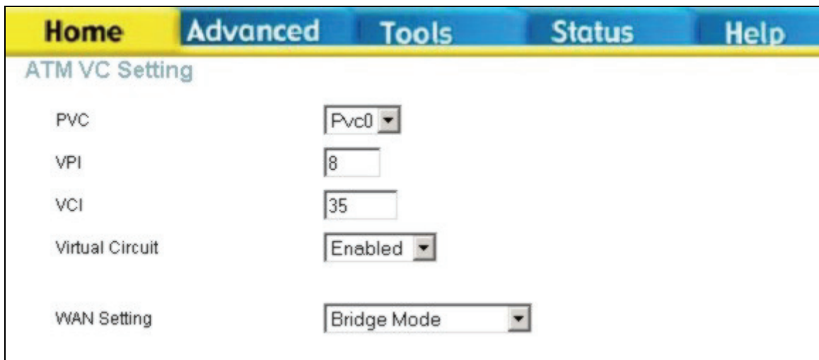
ATM VC Settings in WAN Settings window
