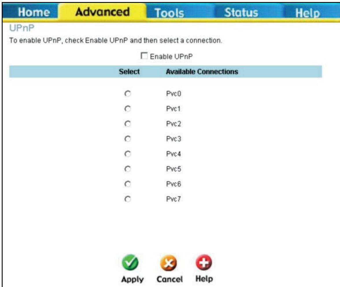
UPnP window
